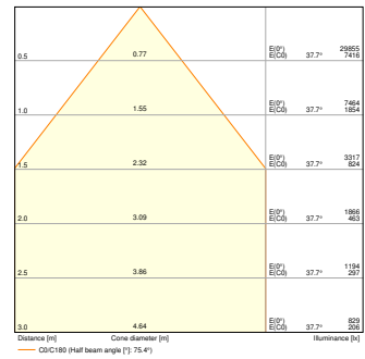
HB P 75W 865 110DEG IP66 PS - REFRACTOR
