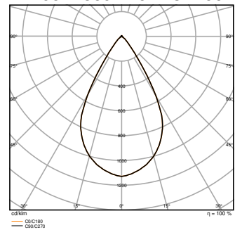
HB P 75W 865 110DEG IP66 PS - REFLECTOR
