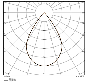
HB P 200W 865 70DEG IP66 PS - REFLECTOR
