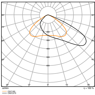
FL FLEX P 360W ML 830 A55X120 WAL LEDV
